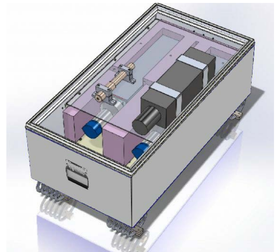
Typical system with 8L Gamma, Neutron and High Dose Detectors
